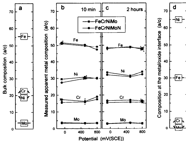
Fig. 13. The composition of the metal phase in at%: (a) the composition of the alloy; (b, c) the apparent composition measured after polarization for 10 min and 2 h, respectively; (d) the estimated composition of the outermost atomic layer of the metal phase under the passive film.
