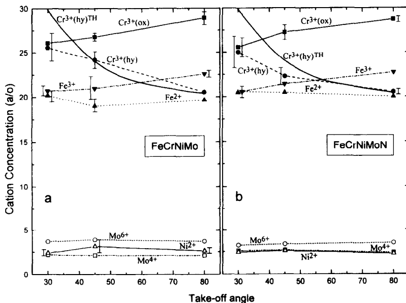
Fig. 7. The cation content in the passive film vs the take-off angle. The solid curves \text{Cr}^{3+}(\text{hy})^{\text{TH}} are theoretical concentrations calculated from a model where a 6.5 Å thick hydroxide layer covers a 10 Å thick oxide.
