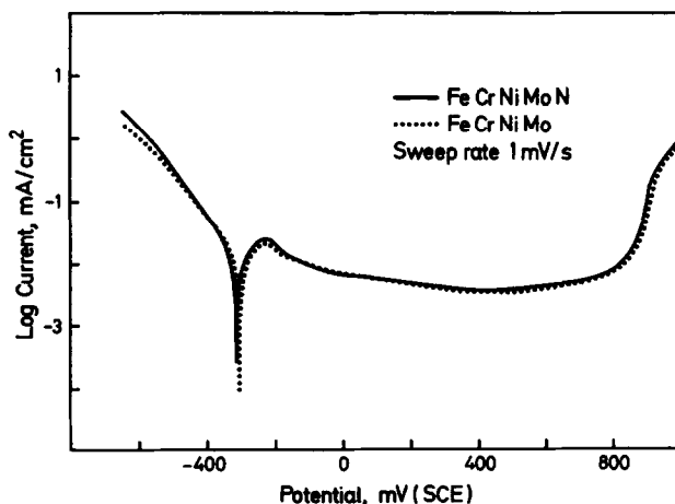
Fig. 1. Potentiodynamic curves for the alloys exposed to de-aerated 0.1 M HCl + 0.4 M NaCl at room temperature, sweep rate 1.0 \text{ mV s}^{-1} .
