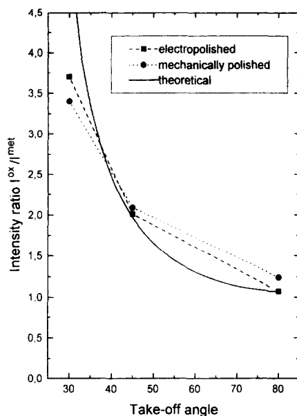
Fig. 6. The measured intensity ratio I^{\text{ox}}/I^{\text{met}} vs the take-off angle after polarization for 10 min at 500 mV (SCE) of an electropolished surface and of a mechanically polished surface.
