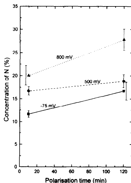
Fig. 10. The coverage of nitrogen at the oxide-metal interface at the potentials -75 , 500 and 800 mV (SCE) for the passivation times 10 min and 2 h.
